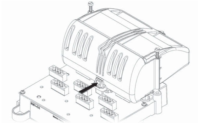
Figure 5.2 - Safety retaining clip for barrier
